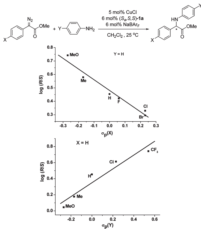
FIGURE 2. The correlations between the log(er) values of the products and the Hammett constants ( \sigma ) of the para substituents.
