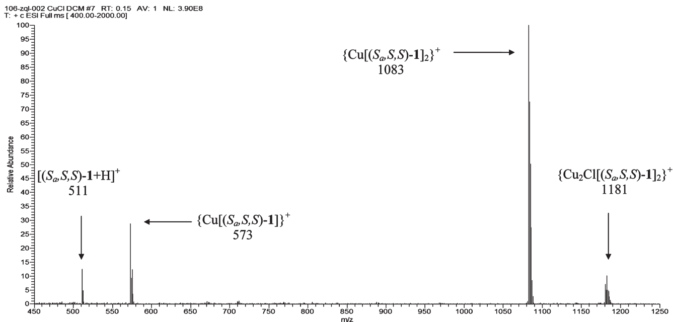
FIGURE 4. ESI-MS analysis of the solution of Cu-( S_a,S,S )- 1a formed by CuCl and ( S_a,S,S )- 1a (1:1 mol) in CH_2Cl_2 .
